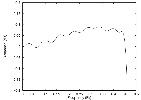
Figure 33 DAC Digital Filter Ripple – 44.1, 48 and 96kHz
