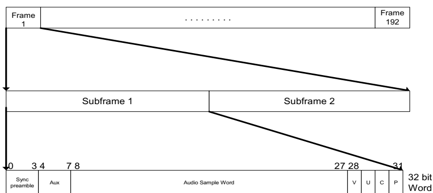
Figure 25 S/PDIF Format
