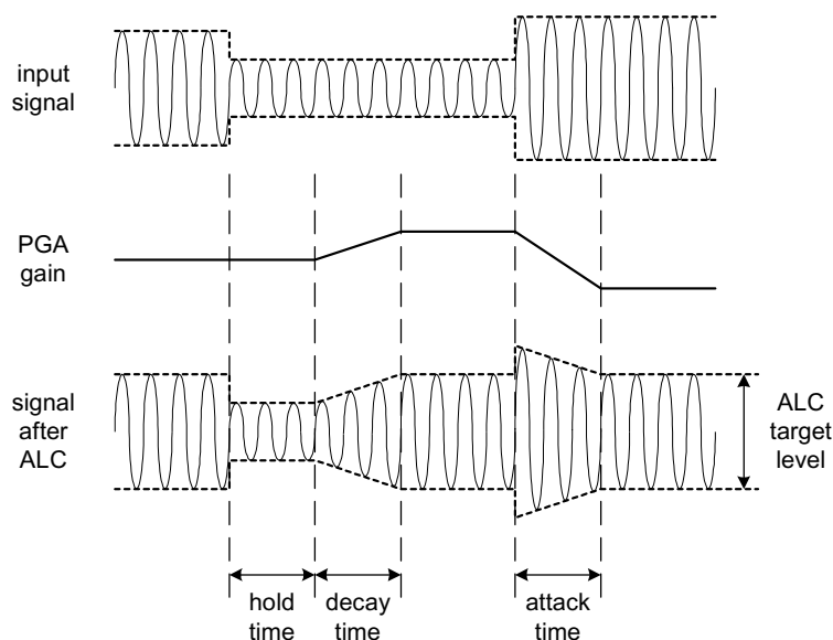
Figure 31 ALC Operation
