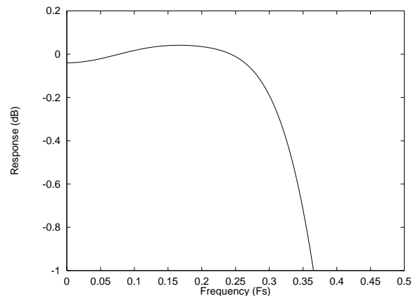
Figure 35 DAC Digital filter Ripple (with DACOSR=1) - 192kHz
